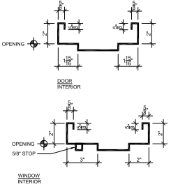
1 DOOR WINDOW FRAME PROFILE 3\" = 1'-0"
