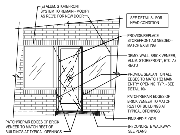
9 DOOR IN EXISTING ALUMINUM STOREFRONT SYSTEM DOOR NO. 128.3 1/4\" = 1'-0"
