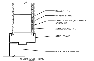
5 DOOR FRAME - FINISHES INTERIOR HEAD (JAMB SIMILAR) 3\" = 1'-0"
